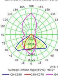
Luminous Intensity Distribution Curve
